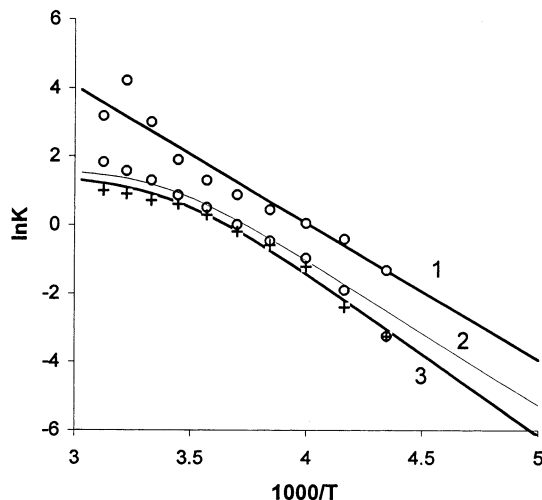
Fig. 27. Van't Hoff plots for spin-crossover of [\text{Fe}(\text{bzimpy})_2] at different pH (1: pH 2.35; 2: pH 7.48; and 3: pH 8.89) calculated using \mu_{\text{HS}} = 5.5 \mu_{\text{B}} .
