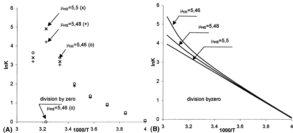
Fig. 28. (A) The effect of different values of \mu_{HS} in transformation of \mu_{obs} to spin–crossover equilibrium constant (experimental data at pH 2.35), and (B) simulated temperature dependencies of K (Eqs. (1.6) and (8.3)).
