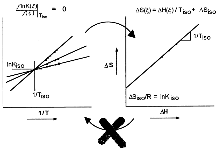
Fig. 2. Left hand side: common point of intersection found for the van't Hoff plots of three reactions belonging to one reaction series (IER, for Arrhenius lines this would correspond to an IKR). Right hand side: linear relationship between entropic and enthalpic contributions to the reactions from the left hand side. If the common point of intersection can be shown with statistical significance, the right hand side can be taken as being implied. However, the reverse argument cannot be granted, because the right hand linear plot might be an artefact without actual physical significance and without implying a common point of intersection at the left hand side.
