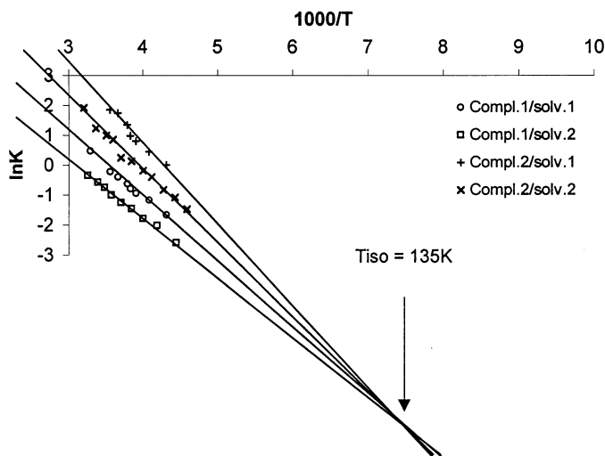
Fig. 18. Isoequilibrium relationship observed in solutions of [\text{Fe}(\text{pyimH})_3](\text{BPh}_4)_2 (complex 1) and [\text{Fe}(\text{PybzimH})_3](\text{BPh}_4)_2 (complex 2 in \text{CH}_3\text{CN}/\text{CH}_3\text{OH} 1:4 (solvent 1) and acetone (solvent 2).
