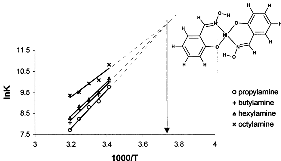
Fig. 23. Isoequilibrium relationship in the series of adducts of bis-(salicylaldoximato)nickel(II) [\text{Ni}(\text{Salcox})_2] with amines.
