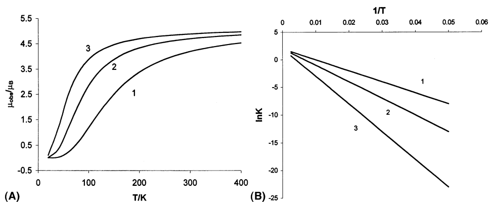
Fig. 15. Isoentropic series of spin-crossover equilibria ( \Delta S/R = 2 , \mu_{HS} = 5.5 ; 1: \Delta H/R = 500 K; 2: \Delta H/R = 300 K; and 3: \Delta H/R = 200 K): A, \mu vs. T curves; B, van't Hoff plots.
