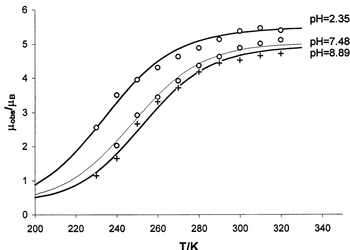
Fig. 25. Temperature dependence of the effective magnetic moment in aqueous methanol solutions of [\text{Fe}(\text{bzimpy})_2](\text{ClO}_4)_2 at different pH. Theoretical curves (lines) are obtained with the same set of parameters shown in Table 5 as corresponding to different pH values.
