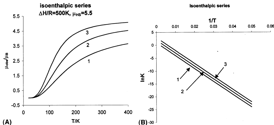
Fig. 14. Isoenthalpic series of spin-crossover equilibria. No intersection point of van't Hoff plots ( \Delta H/R = 500 K, \mu_{HS} = 5.5 ; 1: \Delta S/R = 1 ; 2: \Delta S/R = 2 , and 3: \Delta S/R = 3 ): (A) \mu vs. T curves; (B) van't Hoff plots.
