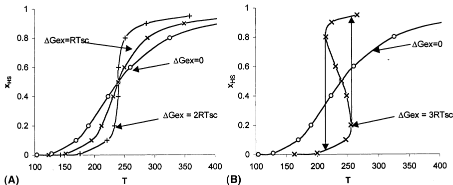
Fig. 10. Shapes of spin-crossover curves. (A) at different values of exchange energy ( \Delta H_{\text{sc}} = 2.5 \text{ kcal mol}^{-1} , T_{\text{sc}} = 240 \text{ K} ) and (B) corresponding to the occurrence of hysteresis.
