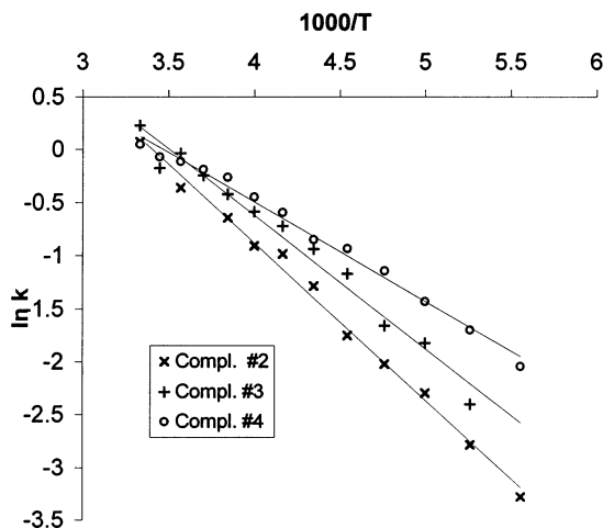
Fig. 5. Arrhenius plots for HS–LS relaxation kinetics in acetone solutions of [\text{Fe}(\text{Py})_3\text{tren}](\text{ClO}_4)_2 of varying concentration.
